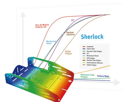
Temperature distribution due to power losses on the component and in the PCB tracks used for solder joint fatigue life estimation. The components in green show no risk of solder joint fatigue; those in yellow show marginal risk. Several design iterations were performed to achieve acceptable lifetime results.
