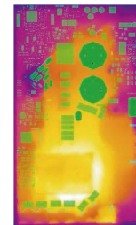
Temperature distribution due to power losses on the component and in the PCB tracks used for solder joint fatigue life estimation. The components in green show no risk of solder joint fatigue; those in yellow show marginal risk. Several design iterations were performed to achieve acceptable lifetime results.
