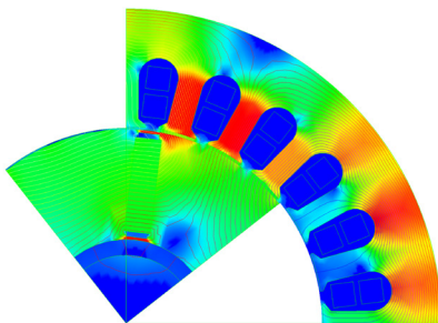
Figure 6. 2D Magnetic fields at 3,000 rpm
