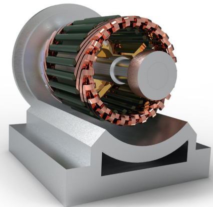
Figure 2. 3D electric motor design mounted on a base – all generated using ANSYS Maxwell
