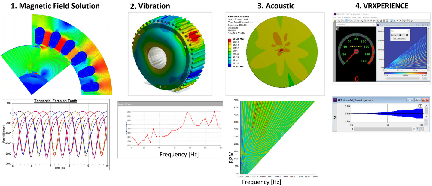
Figure 3. ANSYS NVH solution flow
