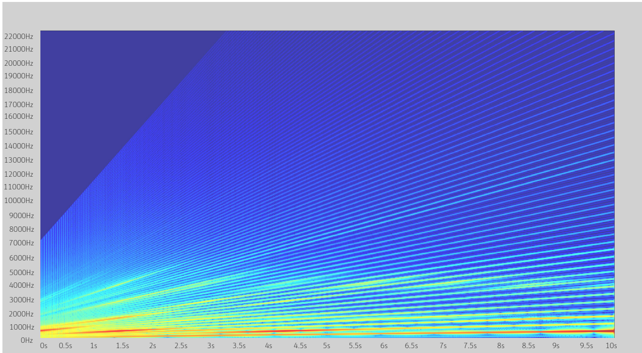
Figure 13. Waterfall diagram for an interior permanent magnet (IPM) motor
