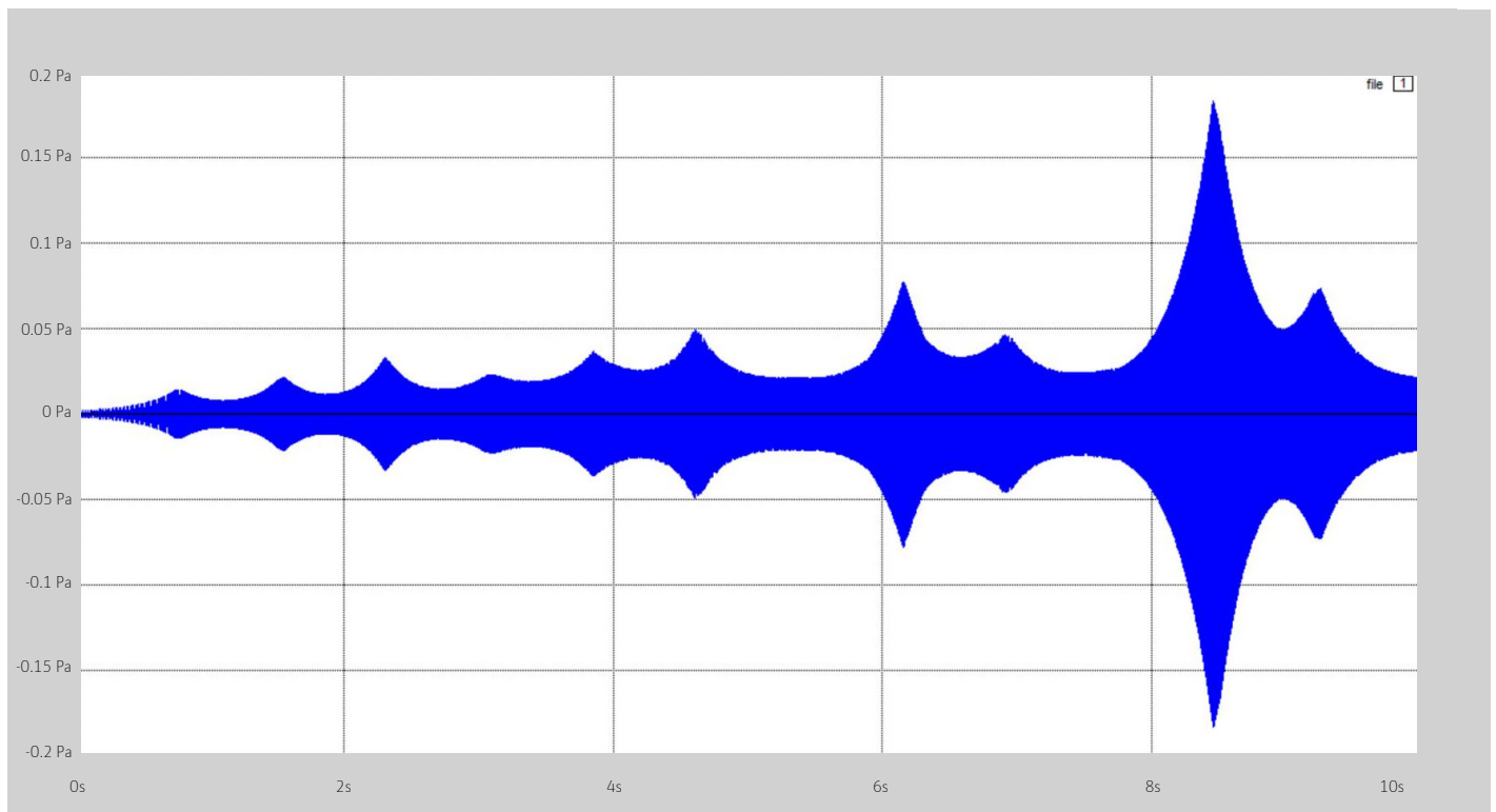
Figure 12. Spectral data displayed in time domain plot
