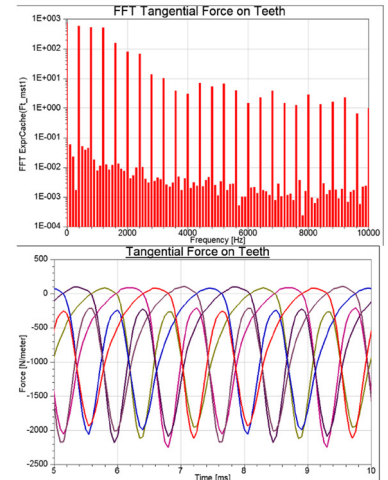
Figure 5. Tangential forces on teeth in ANSYS Maxwell
