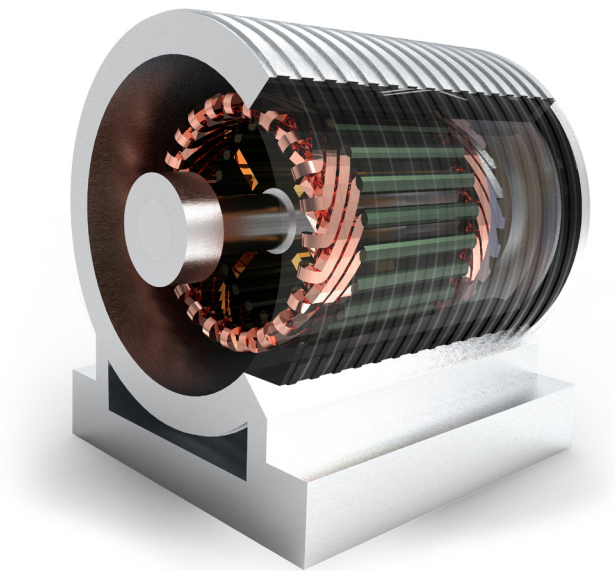
Figure 16. A cut-away view of an electric motor in ANSYS Maxwell
