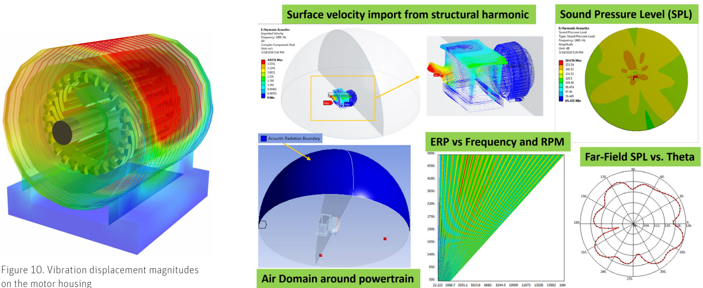
Figure 11. Acoustics and ERP
