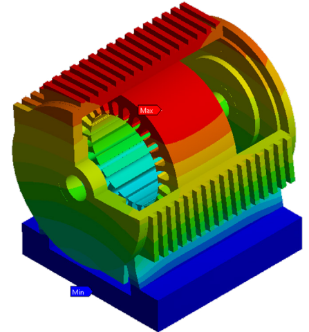
Figure 9. Deformation of the motor in ANSYS Mechanical
